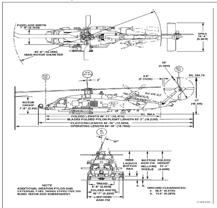
Figure 1-1. Principal Dimensions
